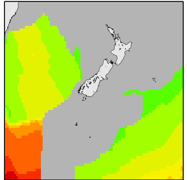
Seafloor Age
