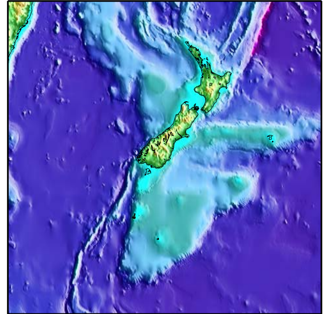
Topography
