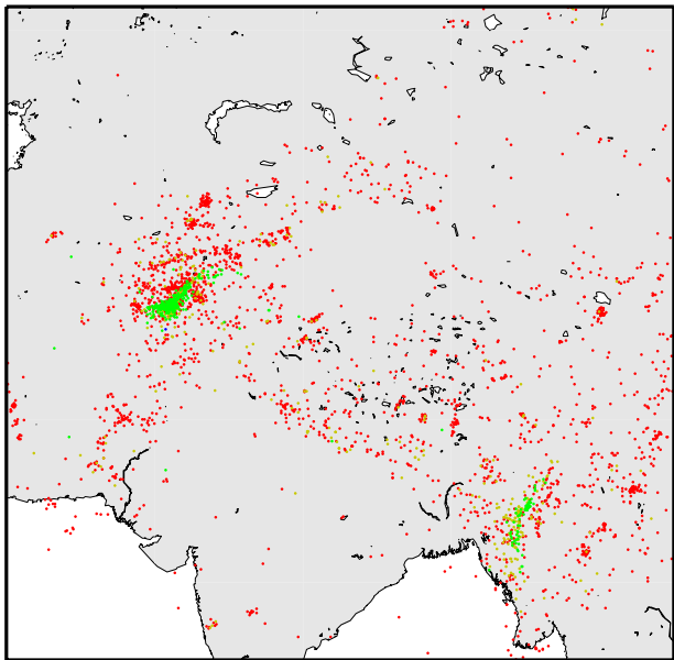
Earthquakes
