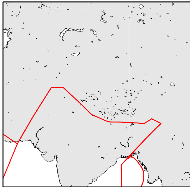
Plate Boundaries
