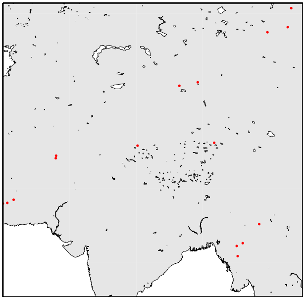
Volcanoes
