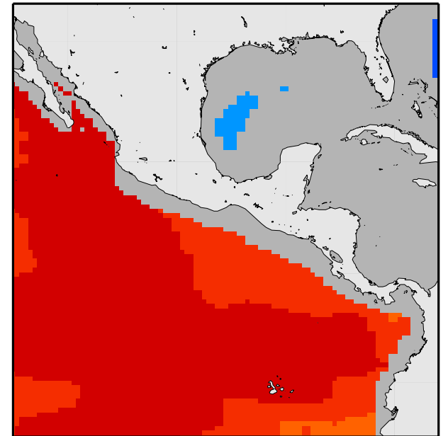
Seafloor Age
