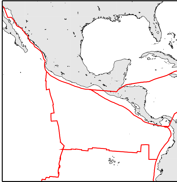
Plate Boundaries
