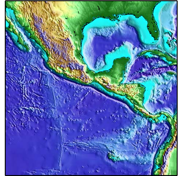
Topography
