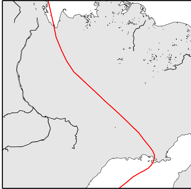
Plate Boundaries
