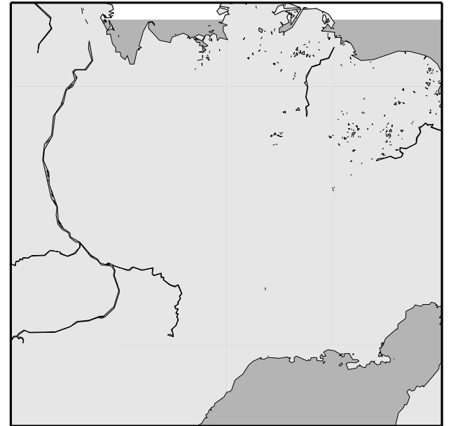
Seafloor Age
