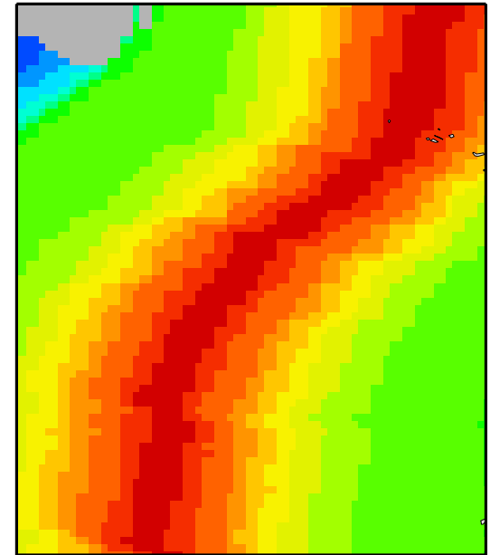
Seafloor Age
