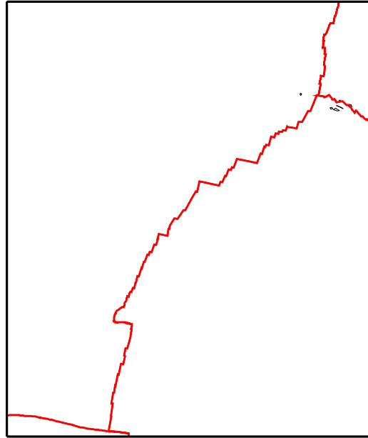
Plate Boundaries
