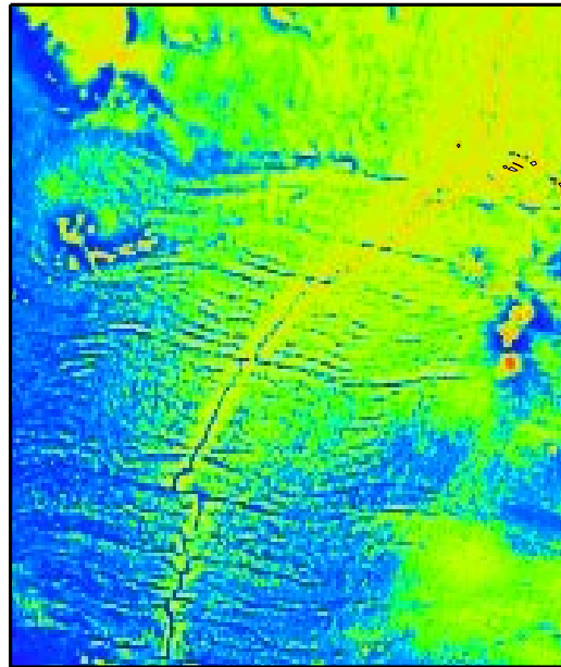
Satellite Gravity
