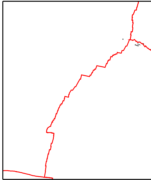
Plate Boundaries
