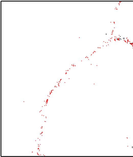
Earthquakes
