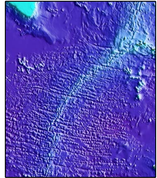
Topography
