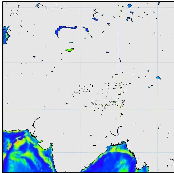
Satellite Gravity
