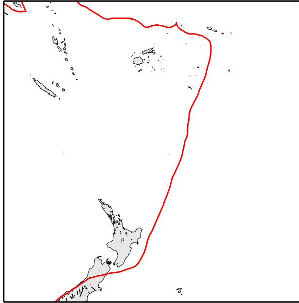
Plate Boundaries
