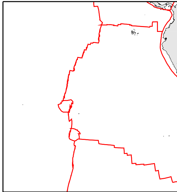
Plate Boundaries
