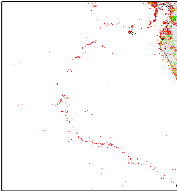
Earthquakes
