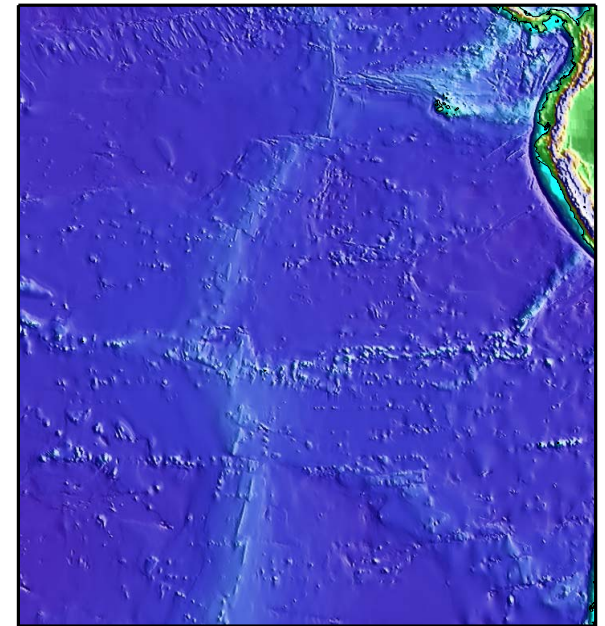
Topography
