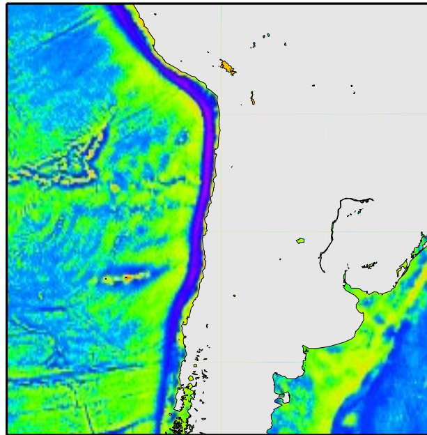
Satellite Gravity
