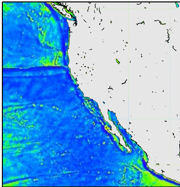
Satellite Gravity
