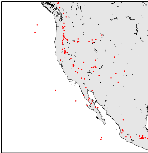
Volcanoes
