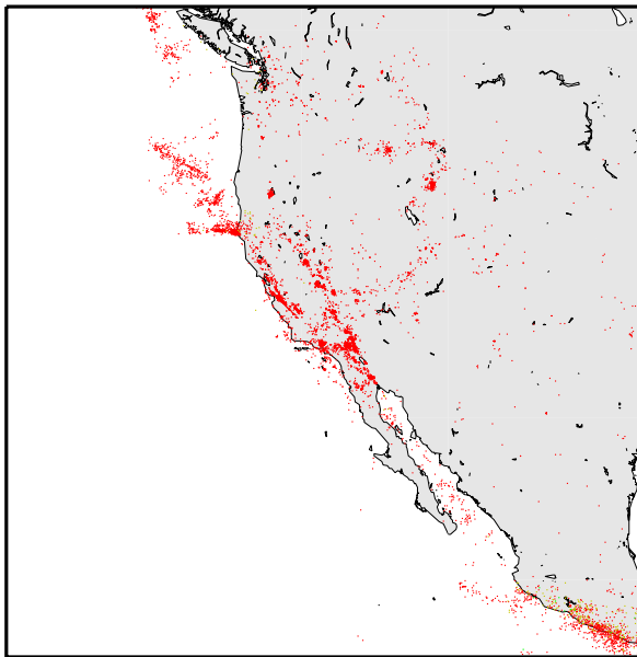
Earthquakes
